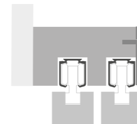
2 BINARI 2 RAILS
