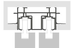
2 BINARI 2 RAILS
