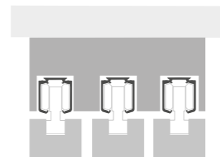
3 BINARI 3 RAILS
